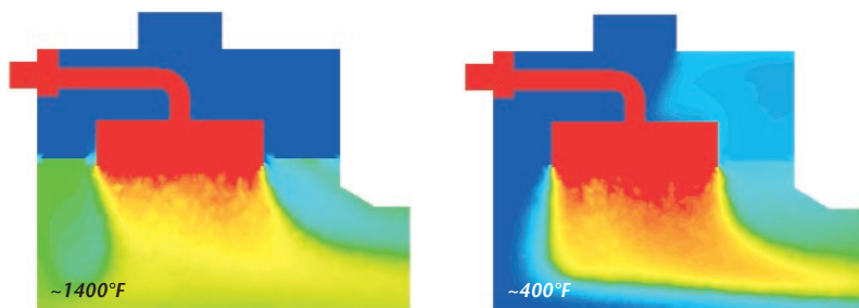
Temperature profiles at cutting planes of X6 with original (left) and modified design (right)
